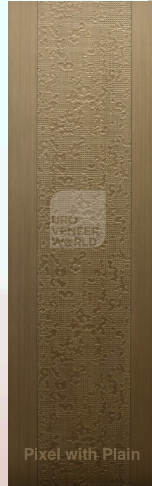
Hybrid 113
